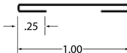
DRIVE CLEAT Model DC
