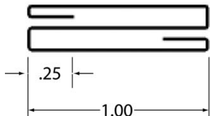
REINFORCED "S" CLEAT Model FSC
