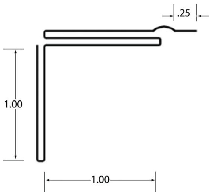
REINFORCED_ STANDING "S" CLEAT Model SSC
