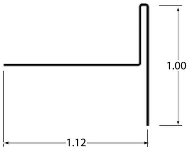
PLASTER GROUND Model PG
