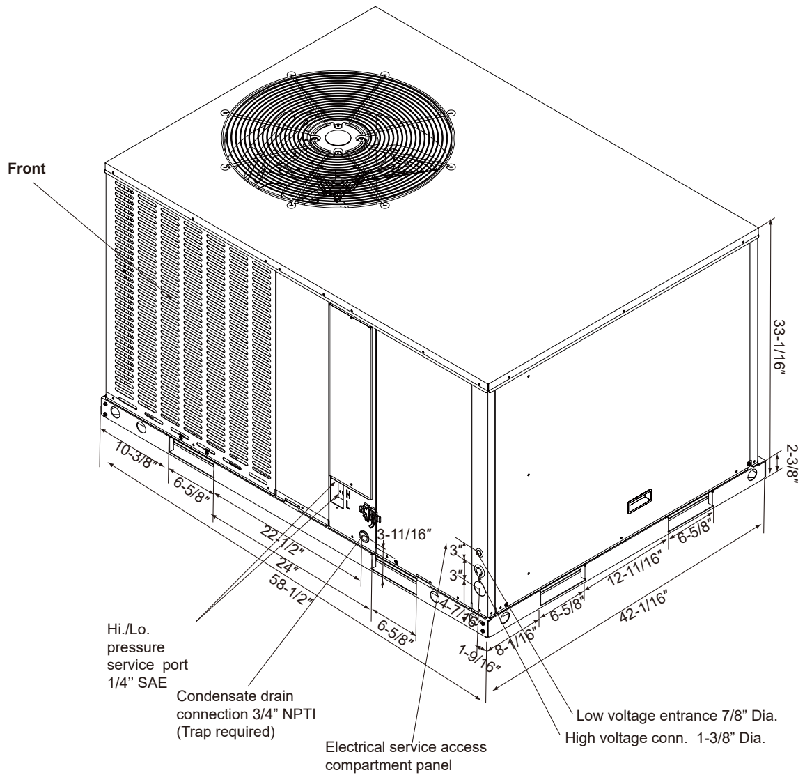
Fig. 2-4 Unit Dimensions
